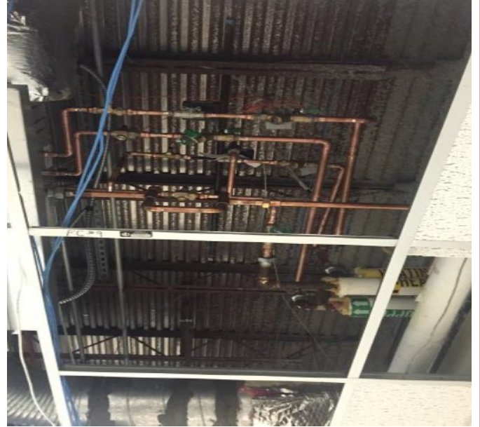
New piping for FCU's at Horace Mann.
